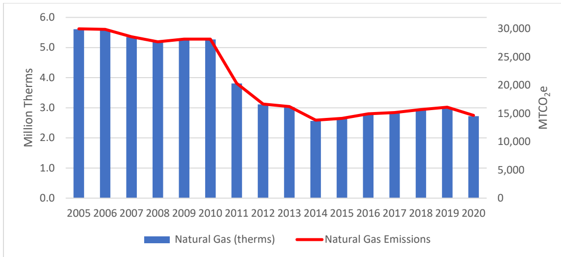
FIGURE 5: NATURAL GAS USE AND EMISSIONS
