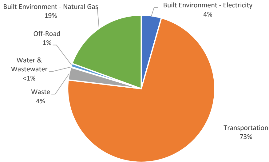
FIGURE 2: EMISSIONS BY SECTOR, 2020
